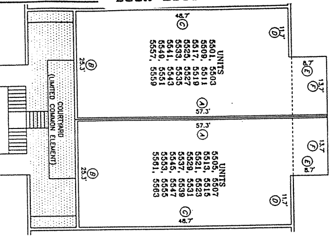
AS-BUILT DIMENSIONS
